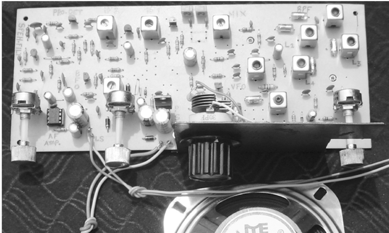
'NSH -1' Assembled Prototype 7 Mhz. AM-SSB-CW Receiver
